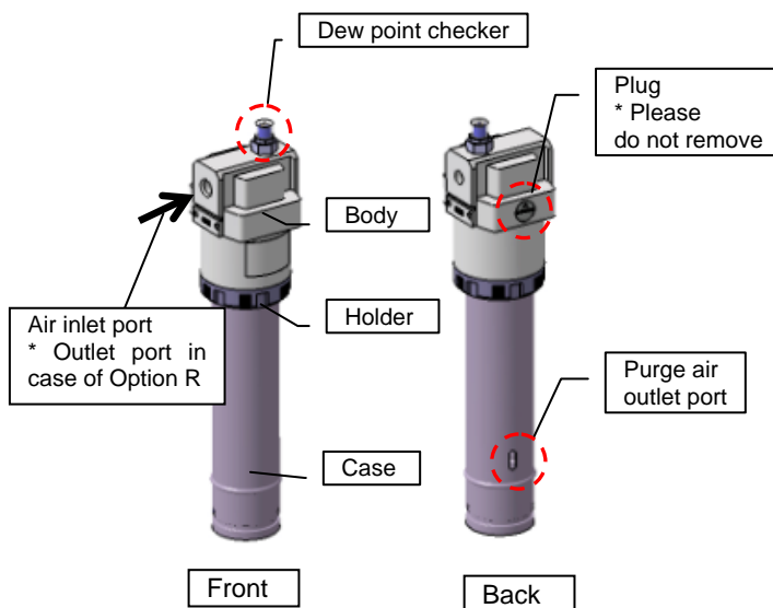
Fig 2.1 Names of parts (Example: IDG30□A)
