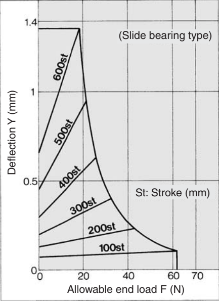
MGCM 32-Stroke-R
