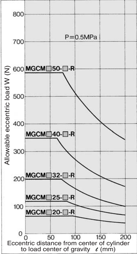
Slide Bearing/ MGCM□□-Stroke-R
