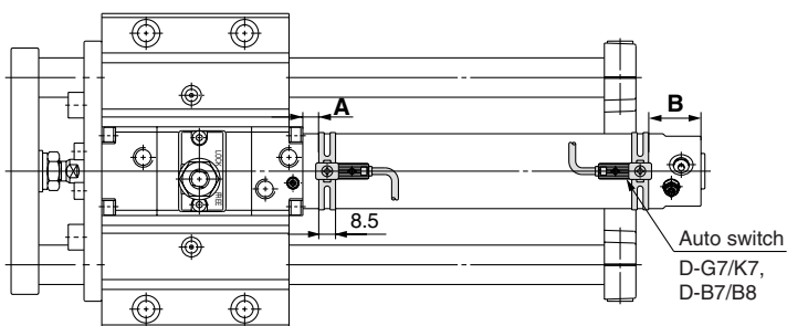
Auto Switch Mounting Height
