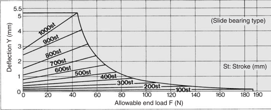
MGCM 50-Stroke-R
