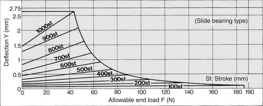
MGCM 50-Stroke-R
