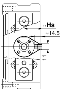
Auto Switch Proper Mounting Position
