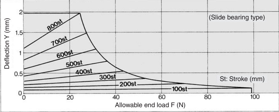
MGCM 40-Stroke-R
