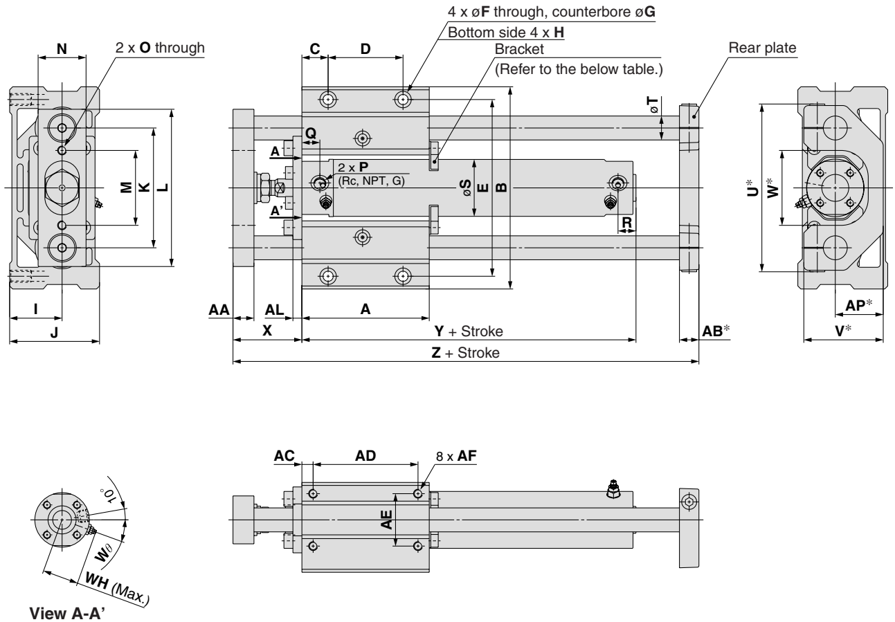
View A-A'
