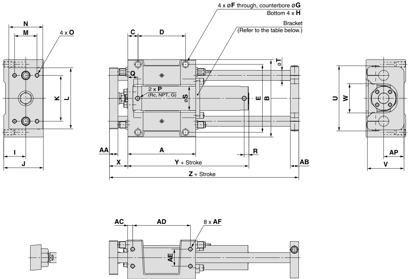
ø100 piston rod end connection
