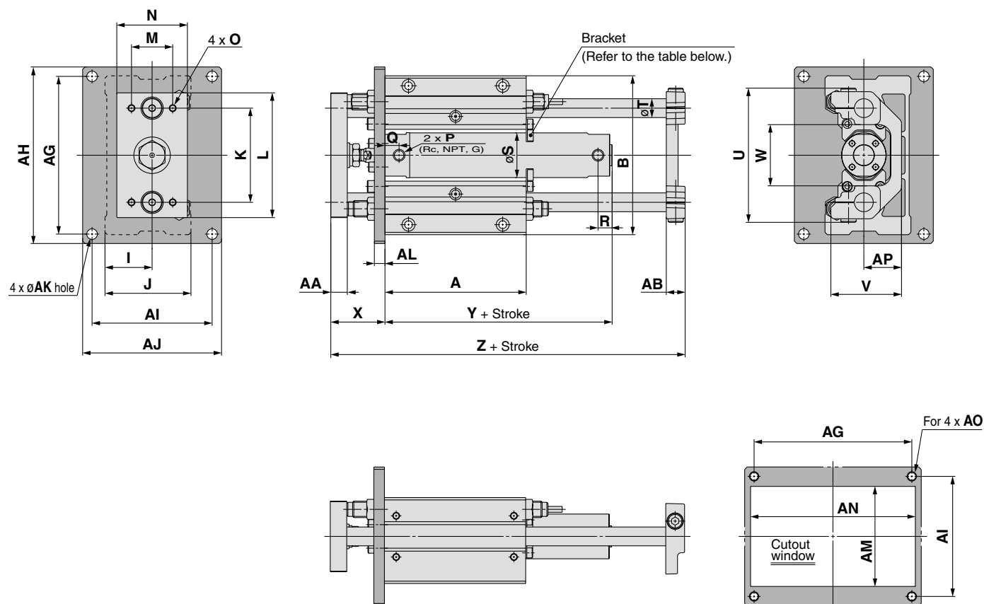
Mounting dimensions
