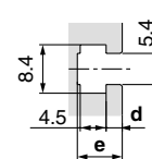
T-slot dimensions (mm)
