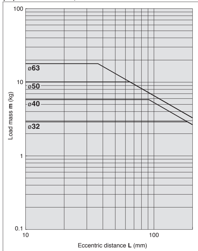
(14) 50 stroke or less, V = 400 \text{ mm/s}
