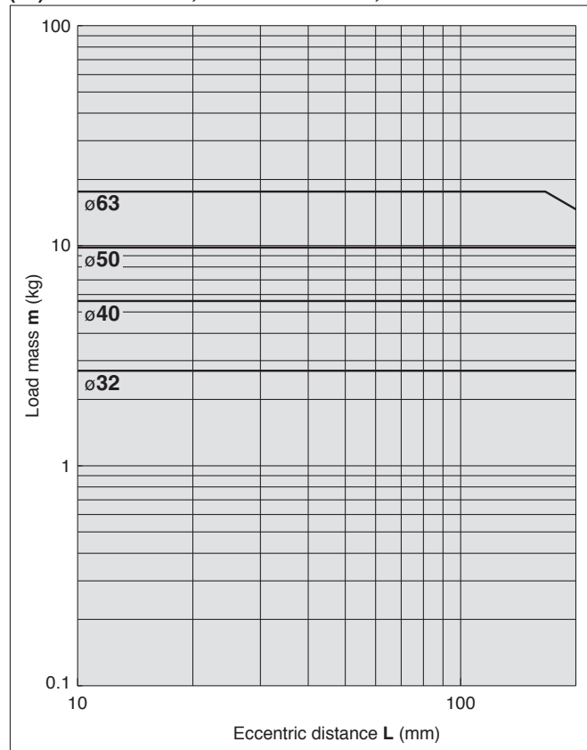
(15) Over 51 stroke, 100 stroke or less, V = 400 \text{ mm/s}
