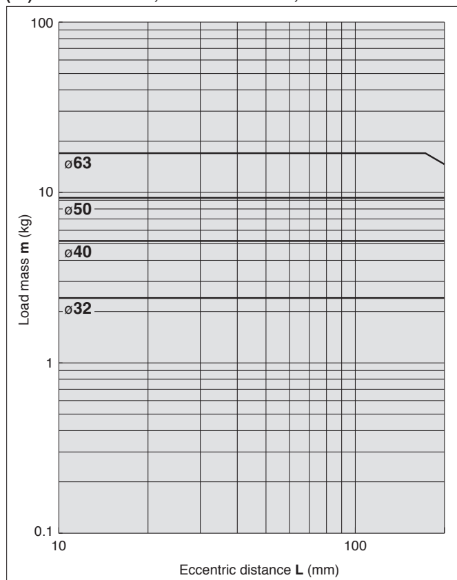
(16) Over 101 stroke, 200 stroke or less, V = 400 \text{ mm/s}
