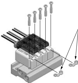
Manifold with more than 3 stations
