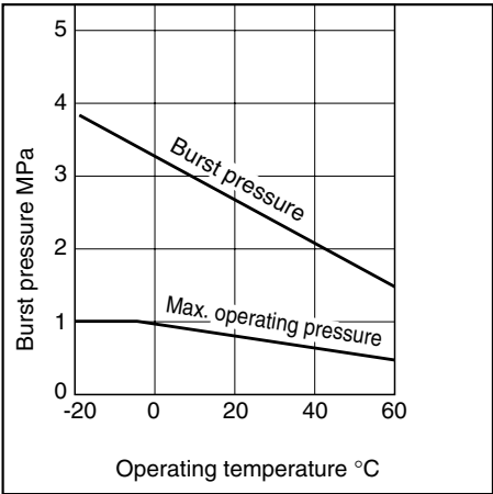
Burst pressure characteristics curve and operating pressure
