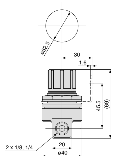
Panel cut dimensions
