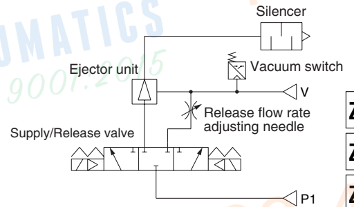
Circuit diagram
