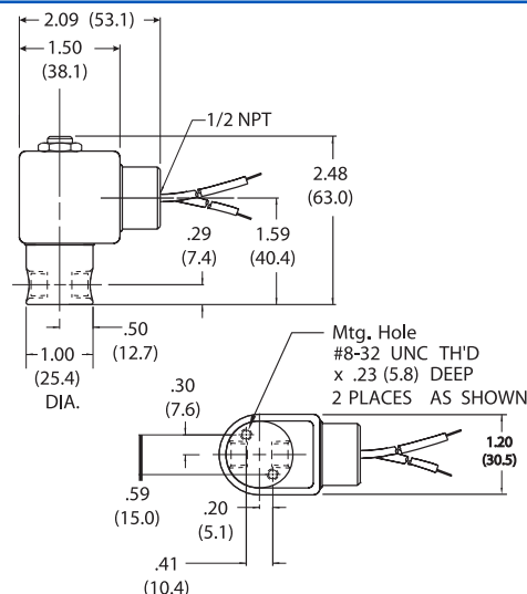
3-Way Normally Closed Exhaust to Atmosphere
