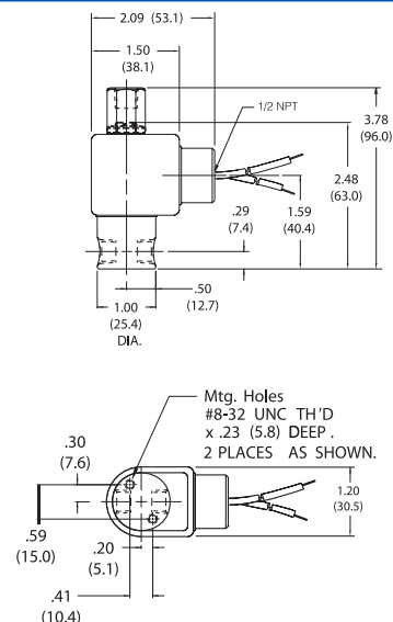
3-Way Normally Closed Piped Exhaust
