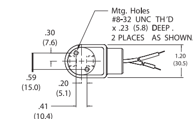
3-Way Styles with Piped Sleeve
